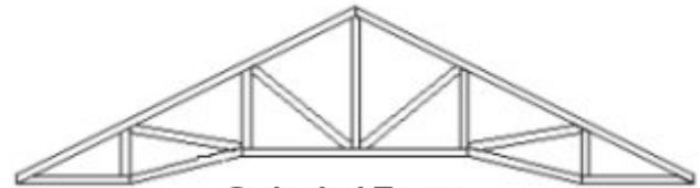
Cathedral Truss
