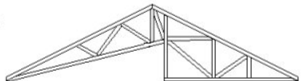
Vaulted Right Truss
