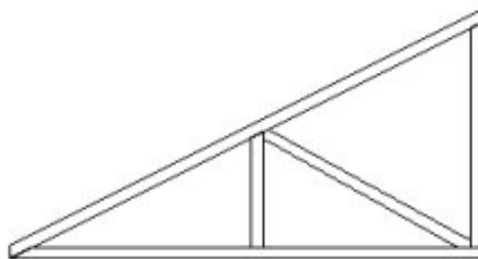
Mono Truss
